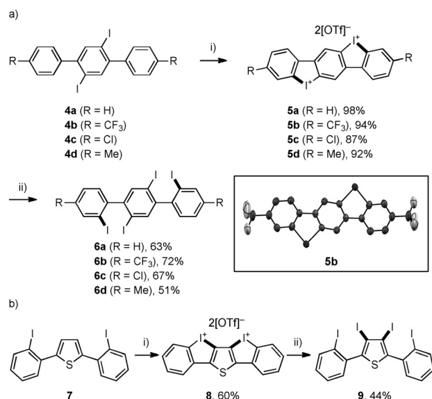
Scheme 3. a) Conversion of 2',5'-diiodo- p -terphenyl derivatives 4a–4d to 2,2',2'',5'-tetraiodo- p -terphenyl derivatives 6a–6d , and b) conversion of 2,5-bis(2-iodophenyl)thiophene 7 to 3,4-diiodo-2,5-bis(2-iodophenyl)thiophene 9 . Reaction conditions: i) m CPBA (3 equiv), TfOH (6 equiv), CH 2 Cl 2 , RT, 2 h; ii) CuI (20 mol%), L1 (40 mol%), [( n Bu) 4 N] + I − (4 equiv), MeCN, 60 °C, 24 h. Inset: ORTEP drawing of 5b (thermal ellipsoids set at 50% probability), whereby hydrogen atoms, counter-anions, and solvent molecules were omitted for clarity.
