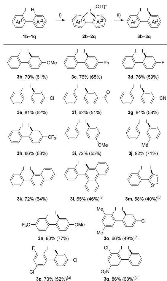
Scheme 2. Two-step conversion of 2-iodobiaryls to 2,2'-diiodobiaryls. Reaction conditions: i) m CPBA (1.5 equiv), TfOH (3 equiv), CH 2 Cl 2 , RT, 1 h; ii) CuI (10 mol %), L1 (20 mol %), [( n Bu) 4 N]I (2 equiv), dioxane, RT, 24 h. The yield refers to that of the second step, and the overall yield over two steps is shown in parentheses. [a] Reaction in DMSO at 60 °C. [b] Reaction in DMF at 60 °C. Tf = trifluoromethanesulfonyl.
