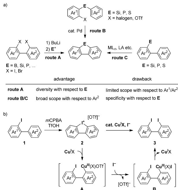
Scheme 1. a) Common synthetic approaches to heterofluorenes (routes A–C) and b) conversion of 2-iodobiaryls to 2,2'-diiodobiaryls through oxidation and iodination ring-opening.
