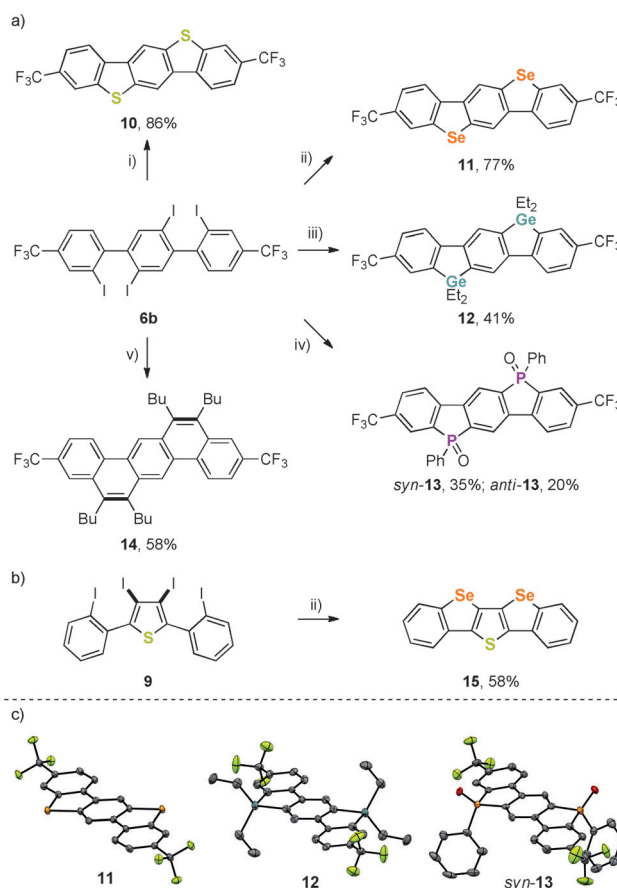
Scheme 4. Conversion of tetraiodoteraryl 6b into ladder-type \pi -conjugated systems. a,b) Reaction conditions: i) CuI (20 mol%), sulfur powder, K 2 CO 3 , DMF, 90 °C; ii) CuI (20 mol%), selenium powder, K 2 CO 3 , NMP, 120 °C; iii) 1) n BuLi, THF, −78 °C; 2) Et 2 GeCl 2 , −78 °C to RT; iv) 1) n BuLi, THF, −78 °C; 2) PhPCl 2 , −78 °C to RT; 3) H 2 O 2 ; v) Pd(OAc) 2 (20 mol%), IPr-HCl (10 mol%), P( t Bu) 3 ·HBF 4 (10 mol%), AgOAc, p -xylene, 130 °C. c) ORTEP drawings of 11 , 12 , and syn - 13 (thermal ellipsoids at 50% probability; hydrogen atoms and solvent molecules were omitted for clarity).
